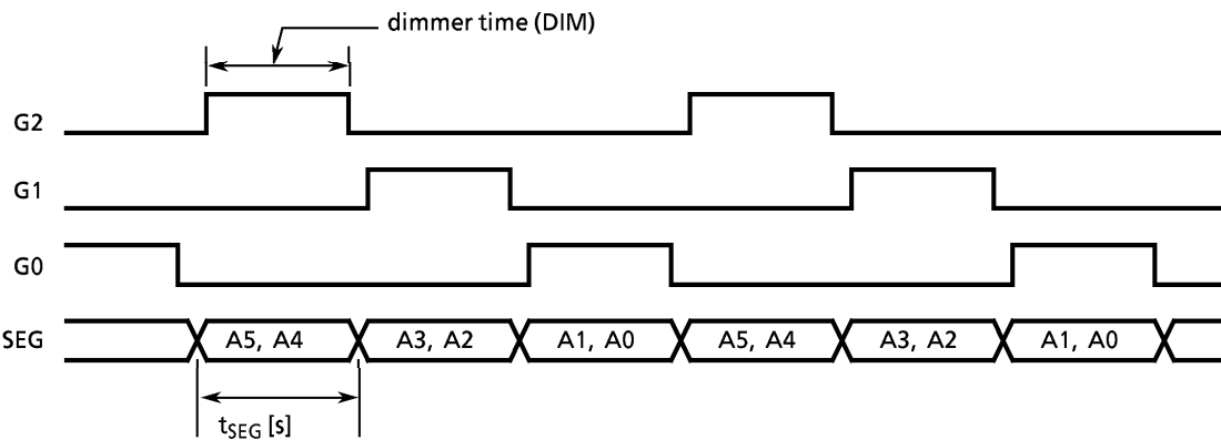
Figure 2-15. VFT drive waveform (3-digit display)
