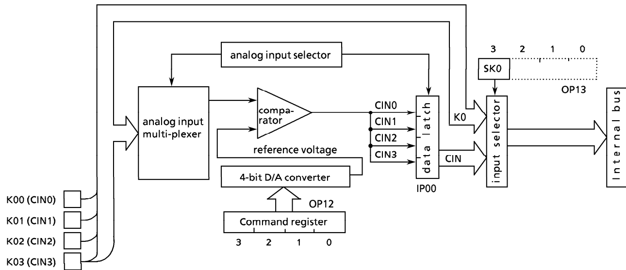
Figure 2-7. Comparator input circuit
