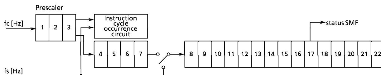
Figure 2-16. Configuration of Timing Generator
