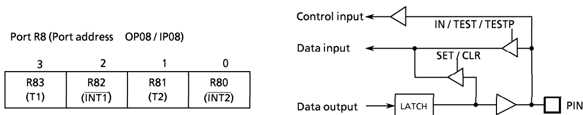
Figure 3-9. Port R8
