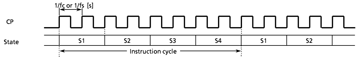
Figure 2-19. Instruction Cycle
