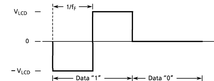
Figure 2-10. LCD drive waveform (COM-SEG pins)
