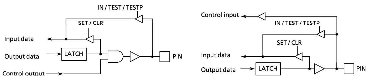
Figure 2-1. port R4
