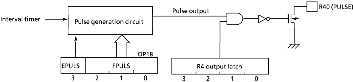
Figure 2-6. Pulse output circuit
