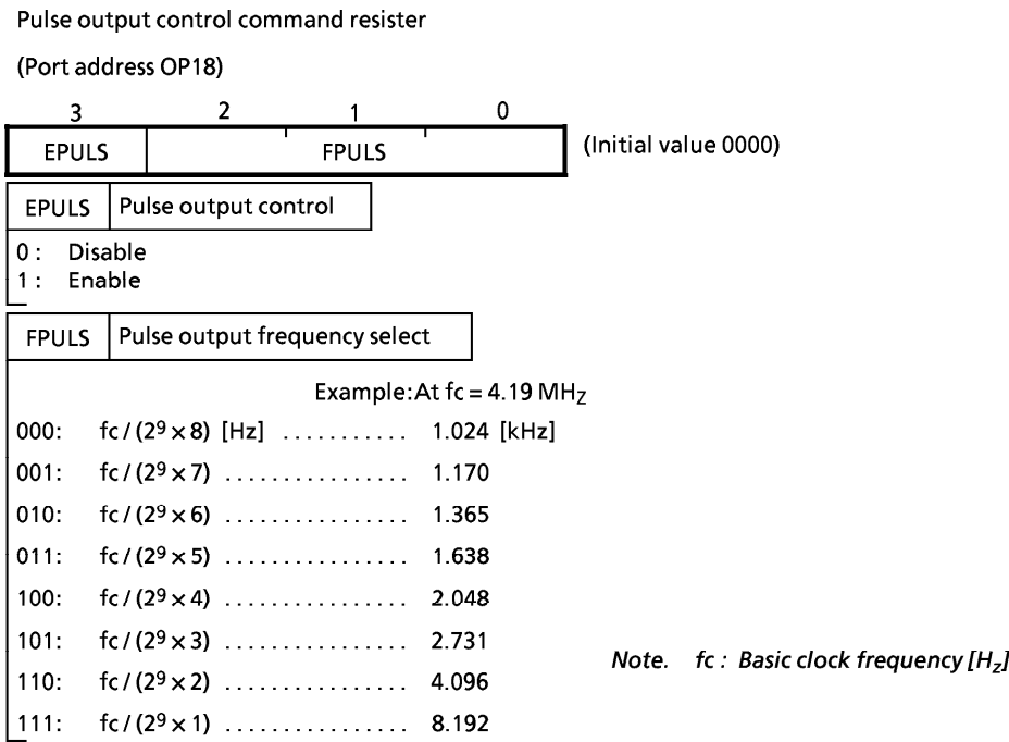
Figure 2-7. Pulse output command register
