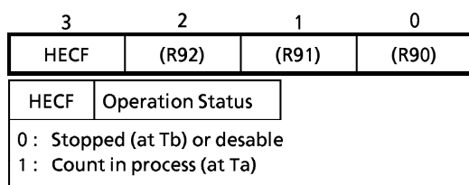
Figure 2-4. HEC Operation status register
