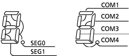
Figure 2-13. Example of COM and SEG connections
