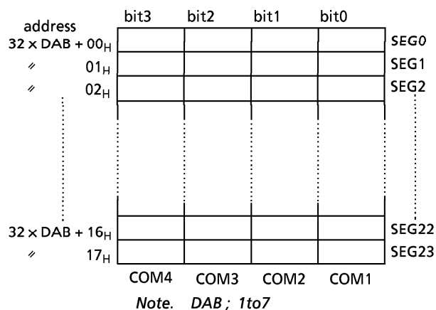
Figure 2-11. The correspondence between the display data area and the SEG/COM pins.
