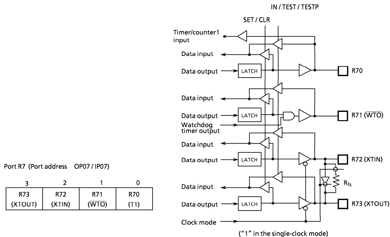
Figure 3-5. Port R7
