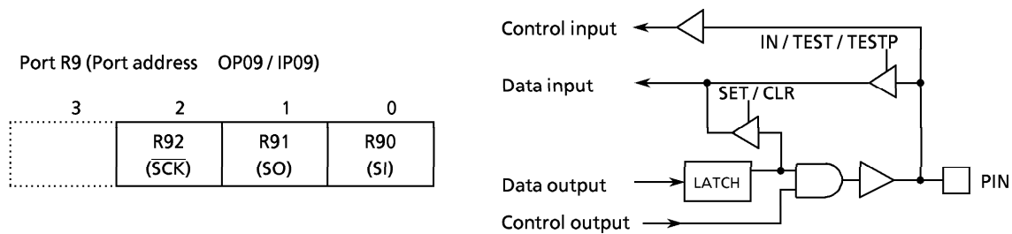
Figure 3-7. Port R9
