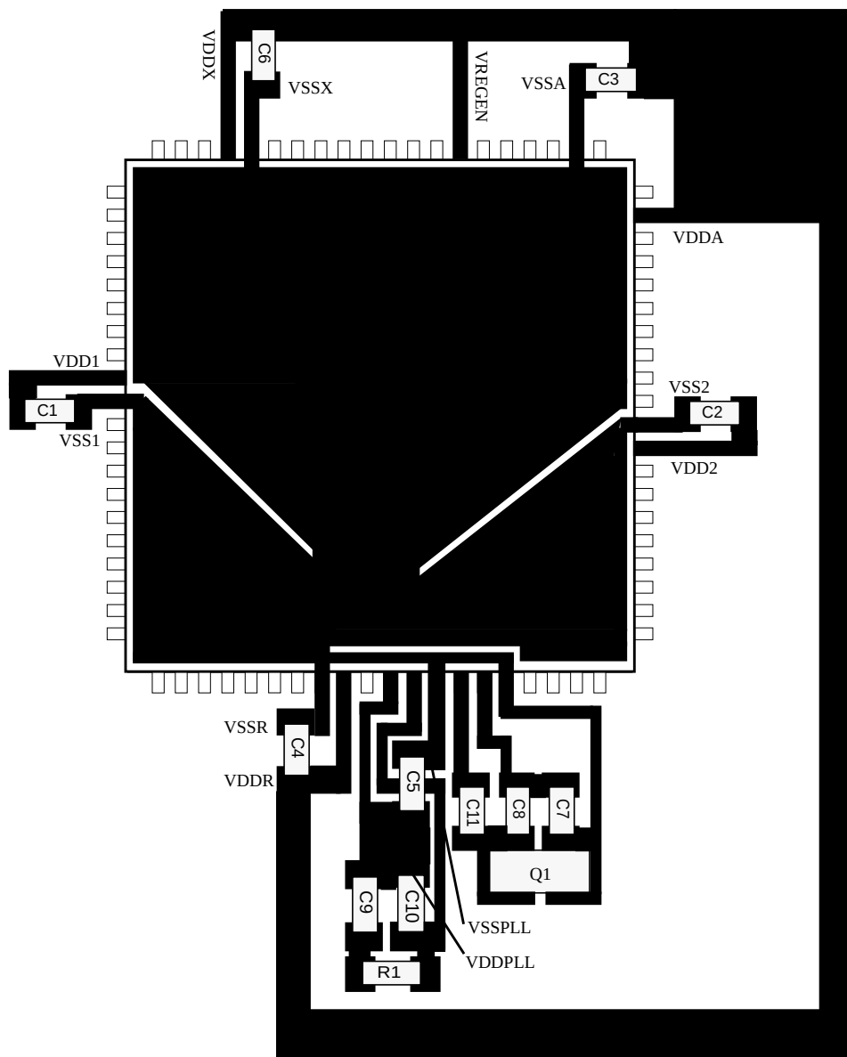
Figure 22-2 Recommended PCB Layout for 80QFP Colpitts Oscillator
