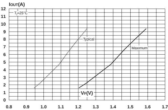
Fig. 7-1: Peak forward voltage drop versus peak forward output current for one power switch at T_J = 25^{\circ}C (typical and maximal values).
