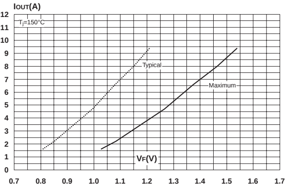
Fig. 7-2: Peak forward voltage drop versus peak forward output current for one power switch at T_J = 150^{\circ}C (typical values and maximal values).
