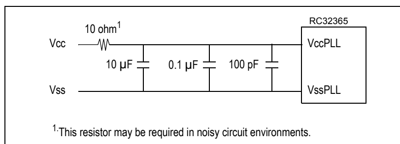
Figure 24 PLL Filter Circuit for Noisy Environments
