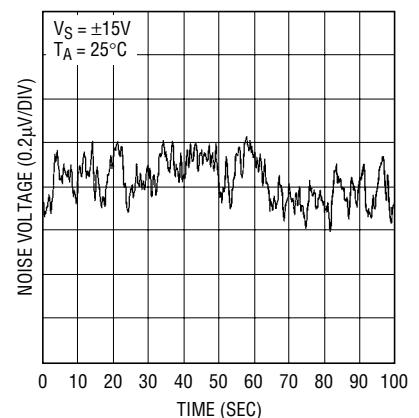
0.01Hz to 1Hz Noise
