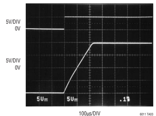
20V Output Step Response
