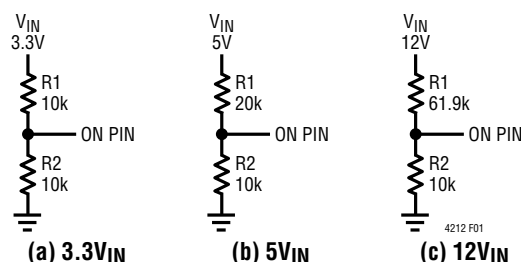
Figure 1. ON Pin Sets the Undervoltage Lockout Voltage Externally
