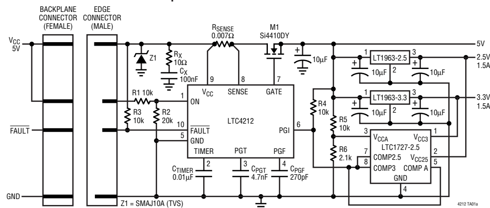
Hot Swap Controller with Power Good Function
