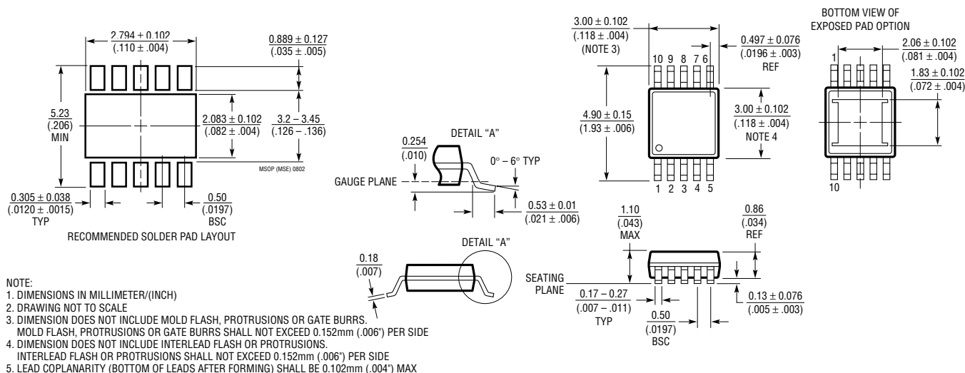
MSE Package 10-Lead Plastic MSOP (Reference LTC DWG # 05-08-1663)
