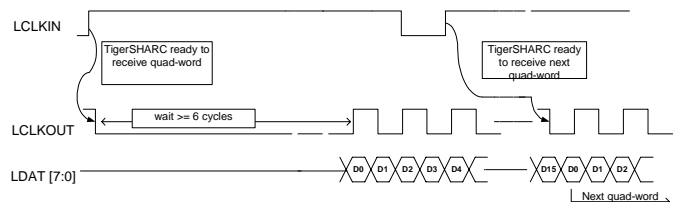
Figure 41. Link Port Data Transfer
