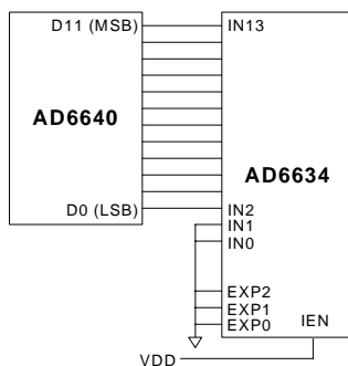
Figure 26. Typical Interconnection of the AD6640 fixed point ADC and the AD6634.
