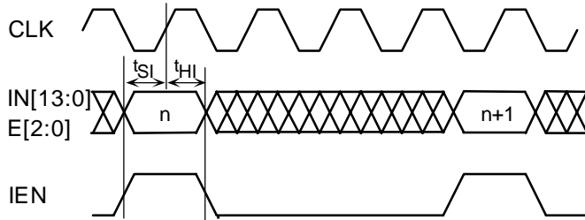
Figure 28. Fractional Rate Input Timing (4X CLK) in mode 01.
