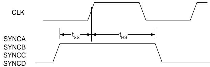
Figure 9. SYNC Timing Inputs
