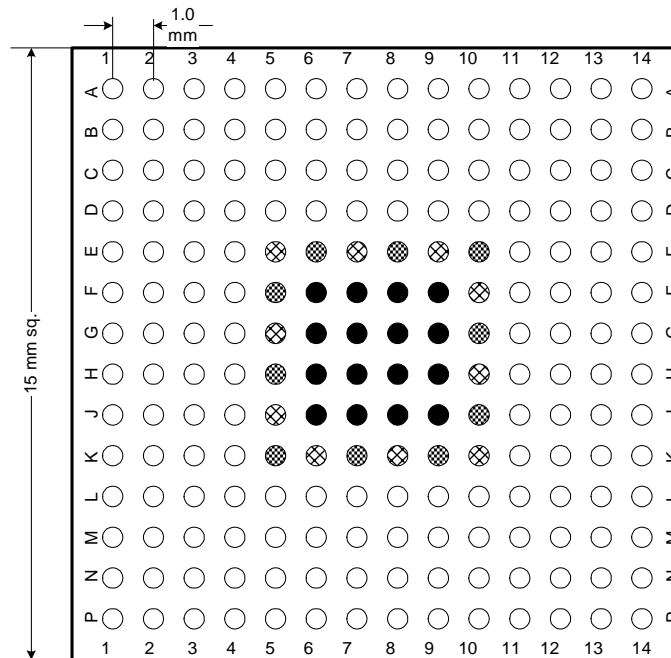
196 Lead BGA (15mm x 15mm) Top View
