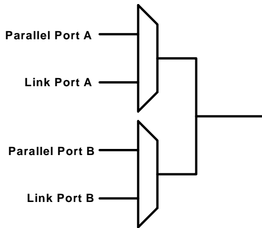
Figure 33 Output port data routing.
