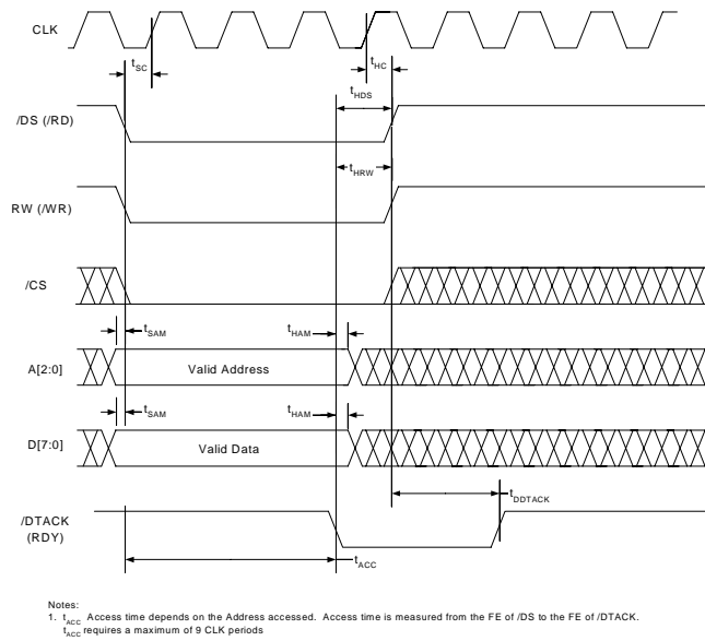
Figure 19. MNM Microport Write Timing Requirements.
