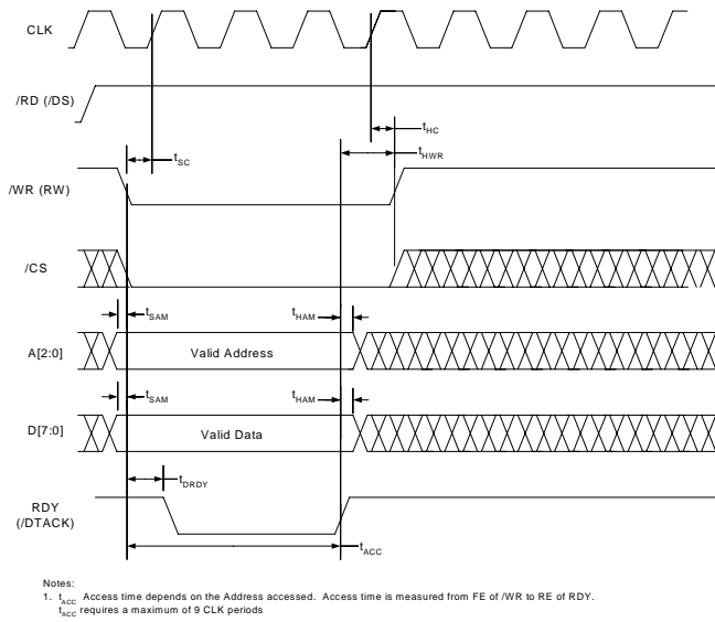
Figure 17. INM Microport Write Timing Requirements.
