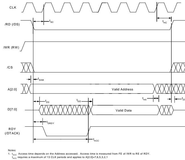
Figure 18. INM Microport Read Timing Requirements.
