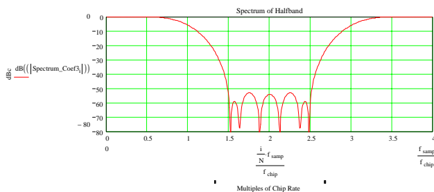
Figure 30. Interpolating Halfband Frequency Response
