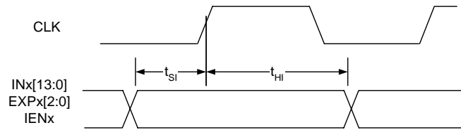
Figure 8. Input Timing for A and B Channels
