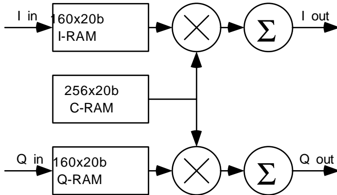
Figure 29. RAM Coefficient Filter Block Diagram
