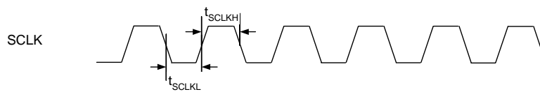
Figure 6. SCLK Switching Characteristics
