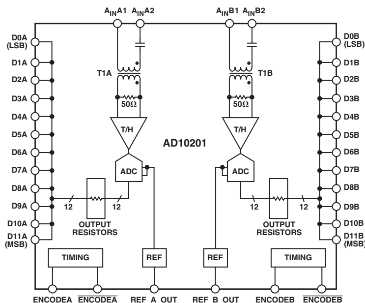
FUNCTIONAL BLOCK DIAGRAM
