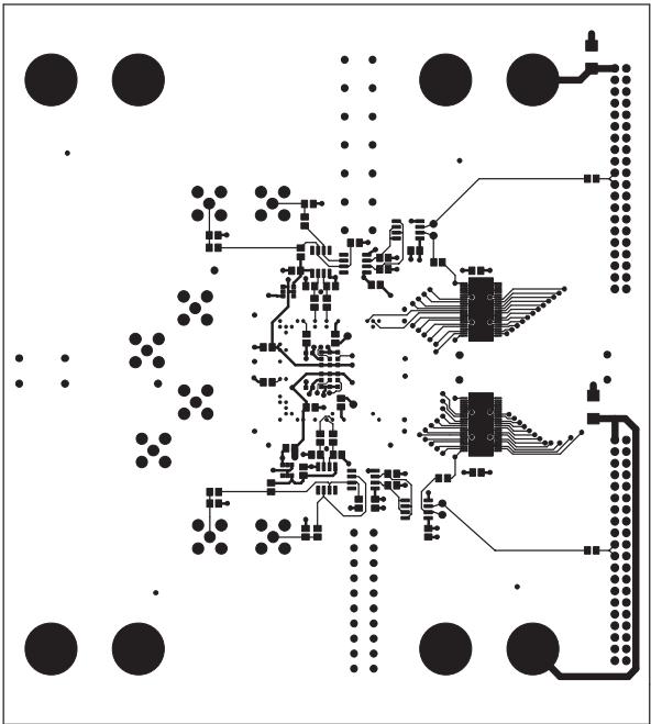
Figure 6c. Top View
