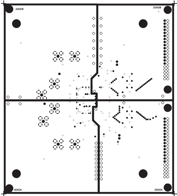
Figure 6f. Bottom View
