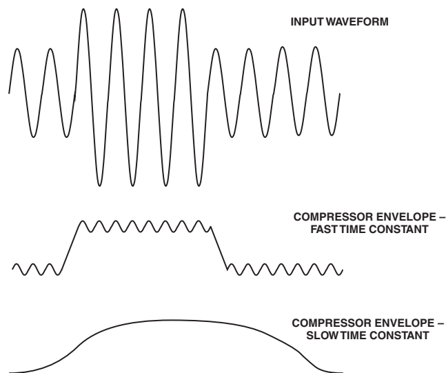
Figure 7. Effect of RMS Time Constant on Distortion
