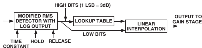
Figure 9. Gain Derived from Interpolated Lookup Table
