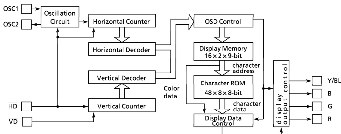
Figure 3-4. OSD Circuit
