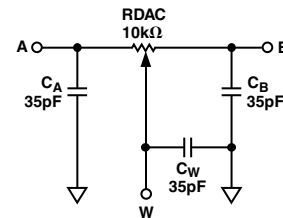
Figure 32. RDAC Circuit Simulation Model for RDAC = 10 kΩ
