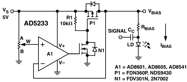
Figure 23. Programmable Booster Voltage Source
