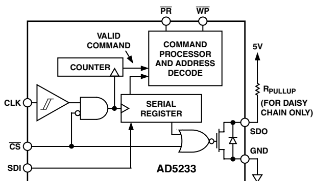
Figure 3. Equivalent Digital Input-Output Logic
