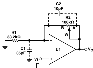
Figure 13. Typical Noninverting Gain Amplifier
