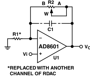
Figure 30. Linear Gain Control with Tracking Resistance Tolerance, and Temperature Coefficient
