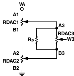
Figure 29. Doubling AD5233 from 6-Bit to 12-Bit
