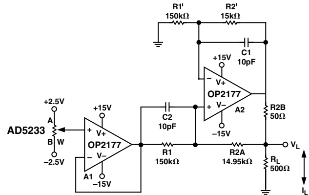
Figure 25. Programmable Bidirectional Current Source
