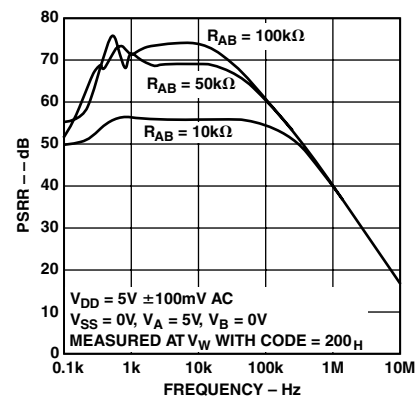
TPC 15. PSRR vs. Frequency
