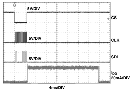
TPC 18. I_{DD} vs. Time (Save) Program Mode
