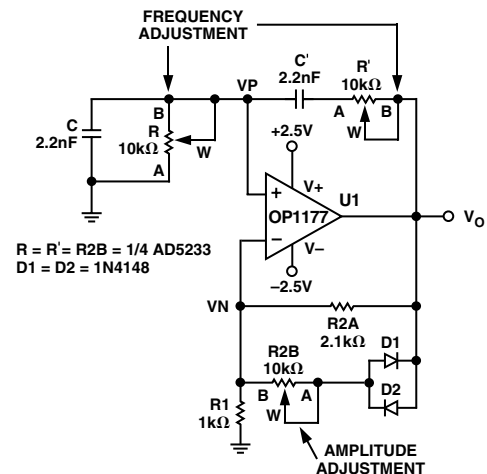
Figure 21. Programmable Oscillator with Amplitude Control
