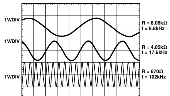
Figure 22. Programmable Oscillation
