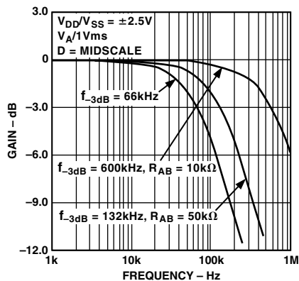
TPC 10. -3 dB Bandwidth vs. Resistance. Test Circuit 7.
