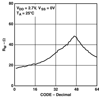
TPC 7. Wiper On-Resistance vs. Code
