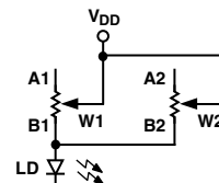
Figure 26. Reduce Resistance by Half with Linear Adjustment Characteristics
