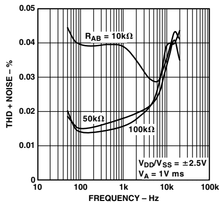
TPC 11. Total Harmonic Distortion vs. Frequency
