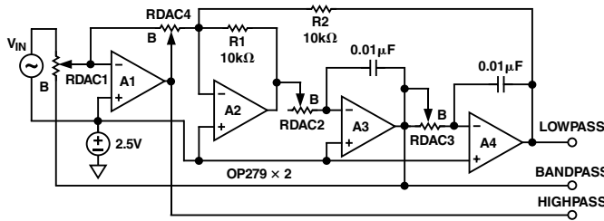
Figure 18. Programmable Stable Variable Filter
