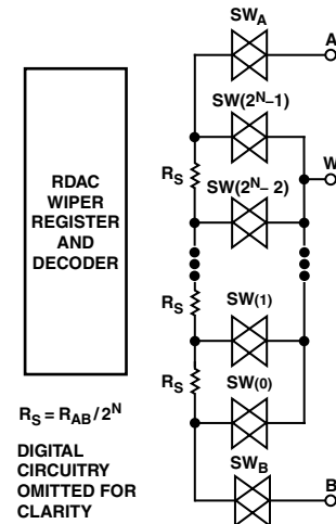
Figure 9. Equivalent RDAC Structure (Patent Pending)
