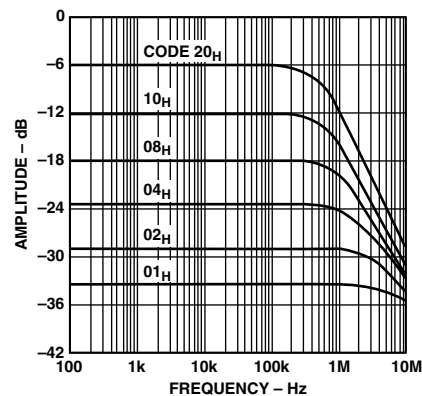
TPC 12. Gain vs. Frequency vs. Code, R_{AB} = 10 \Omega . Test Circuit 7.
