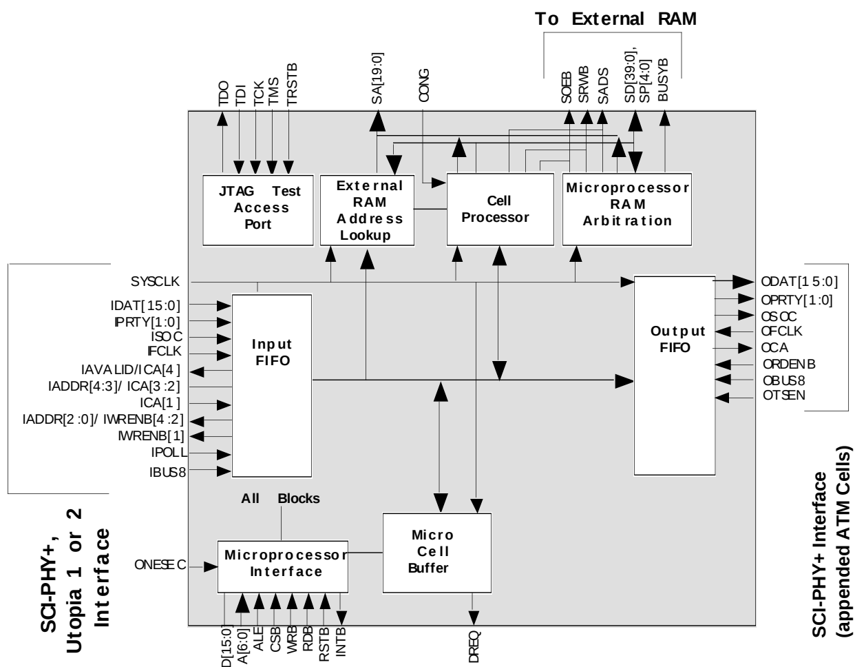
Fig. 2 Block Diagram
