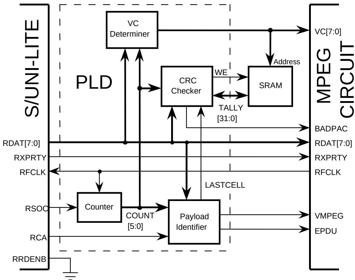
Figure 1 - S/UNI-LITE Interfacing with CATV Headend MPEG Circuitry
