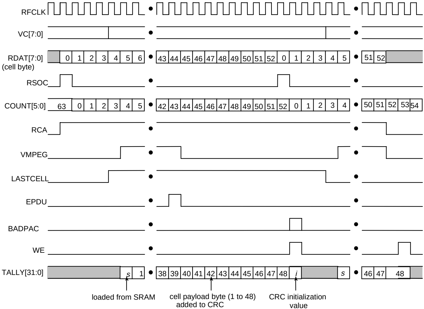
Figure 2 - Functional Timing of S/UNI-LITE to MPEG Circuitry
