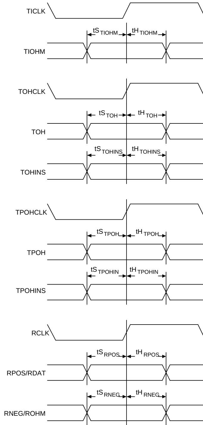
Figure 50 - Input Timing
