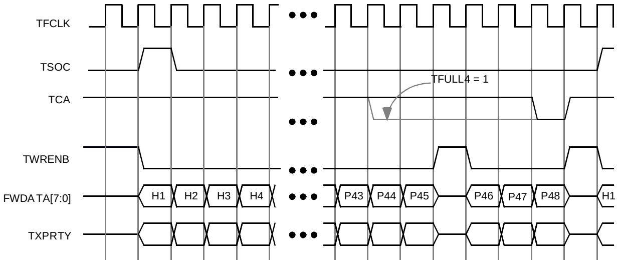
Figure 39 - Transmit Synchronous FIFO (100-pin PQFP with SYFIFOB=0)
