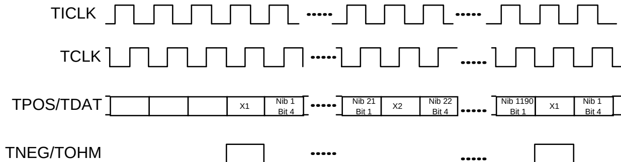
Figure 27 - Transmit Unipolar DS3 Stream
