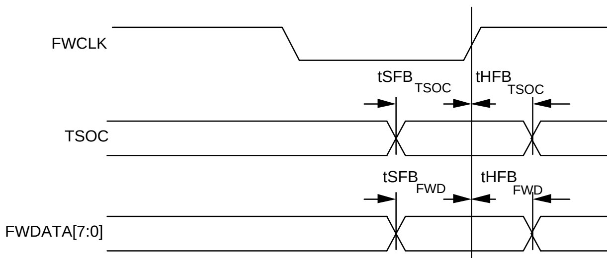
Figure 48 - Transmit System Side - FIFO Bypass
