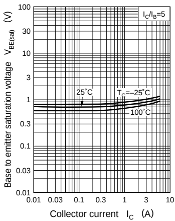
V_{BE(\text{sat})} - I_C
