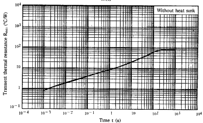
R_{th(t)} - t
