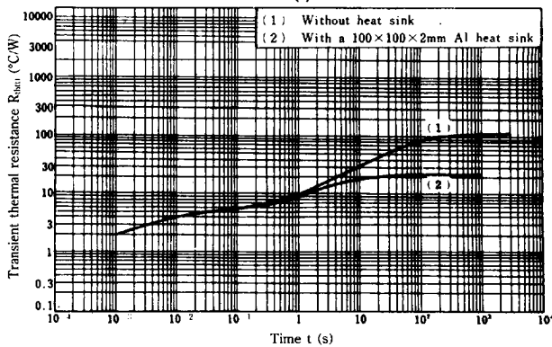
R_{th}(t) - t
