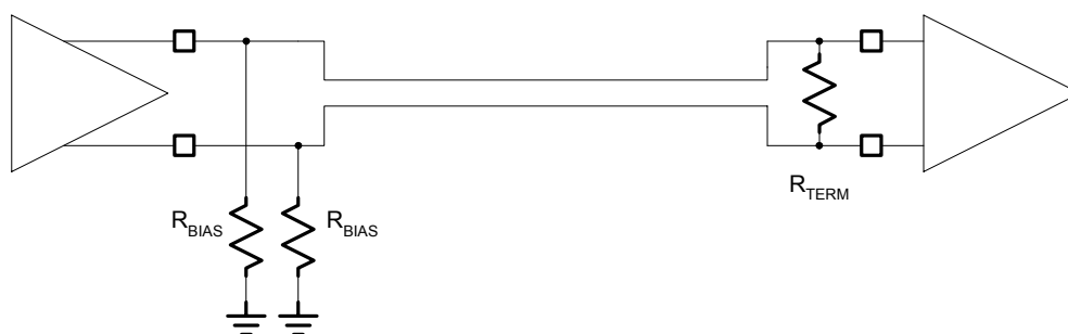
FIGURE 1. PECL INTERFACE
