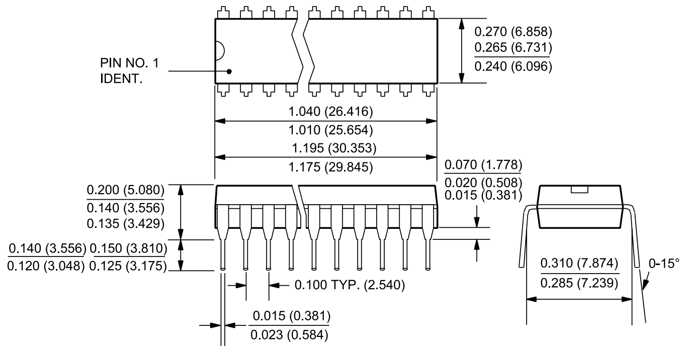
20-Pin DIP
