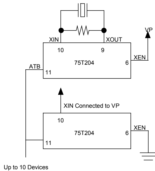
FIGURE 2: Crystal Connections
