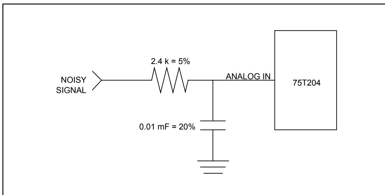
FIGURE 5: RC Filter
