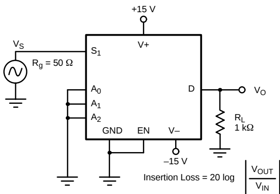
FIGURE 8. Insertion Loss
