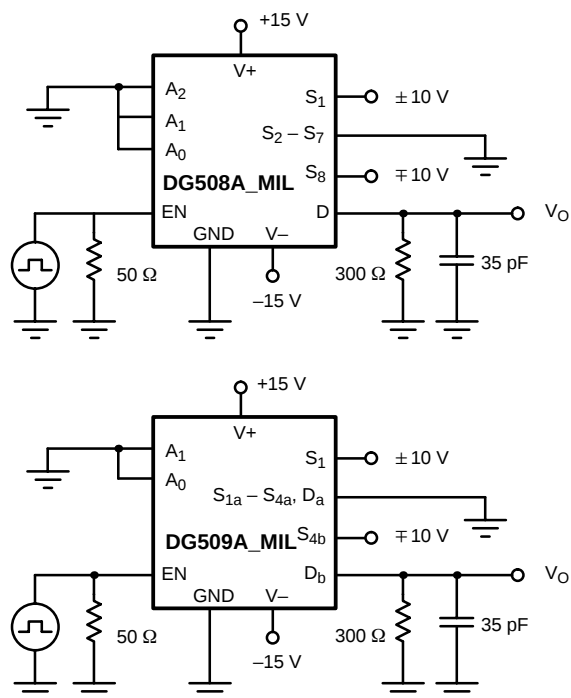
FIGURE 2. Transition Time
