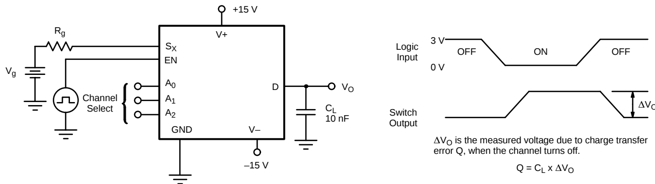
FIGURE 5. Charge Injection
