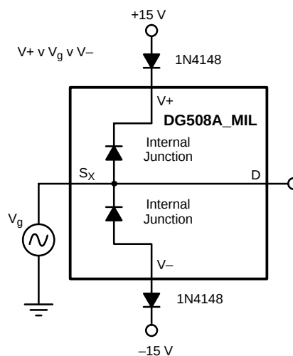
FIGURE 10. Overvoltage Protection Using Blocking Diodes
