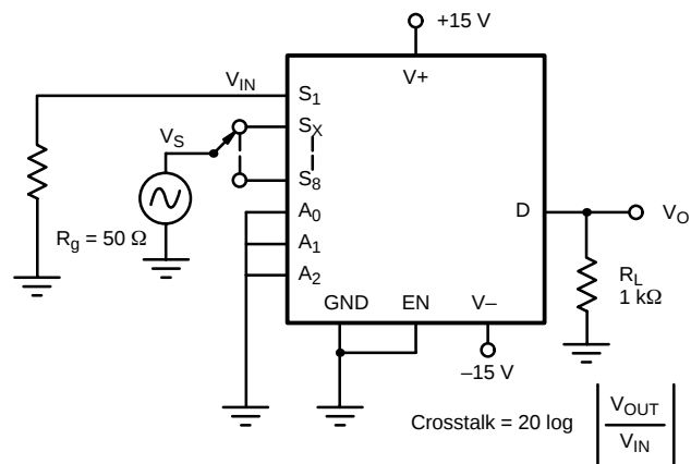
FIGURE 7. Crosstalk
