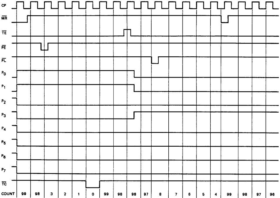
Fig.6 Timing diagram.
