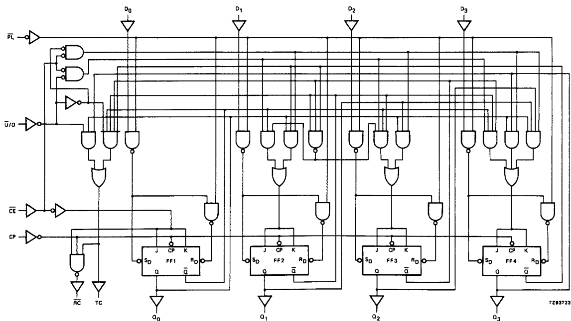
Fig.9 Logic diagram.
