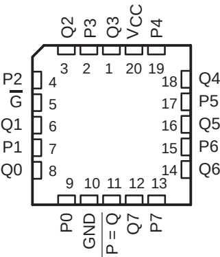
54ACT11521 . . . FK PACKAGE (TOP VIEW)
