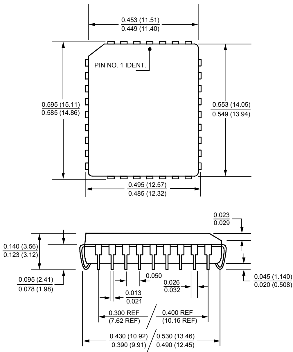
32-Pin PLCC
