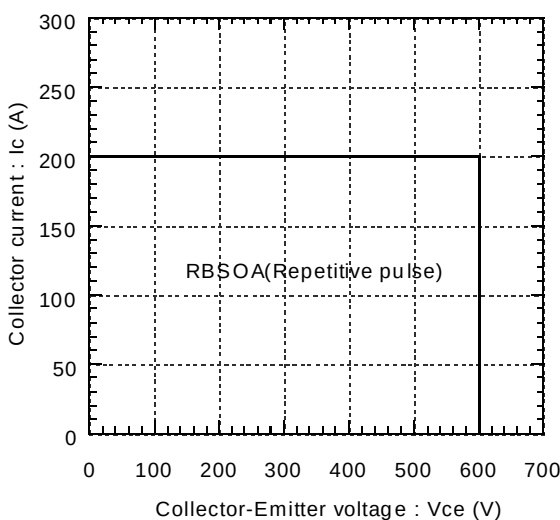
Reversed biased safe operating area Vcc=15V,Tj≤25°C
