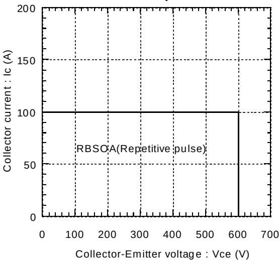
Reversed biased safe operating area V_{cc}=15\text{V}, T_j \leq 25^{\circ}\text{C}
