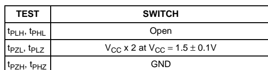
FIGURE 7. AC Test Circuit
