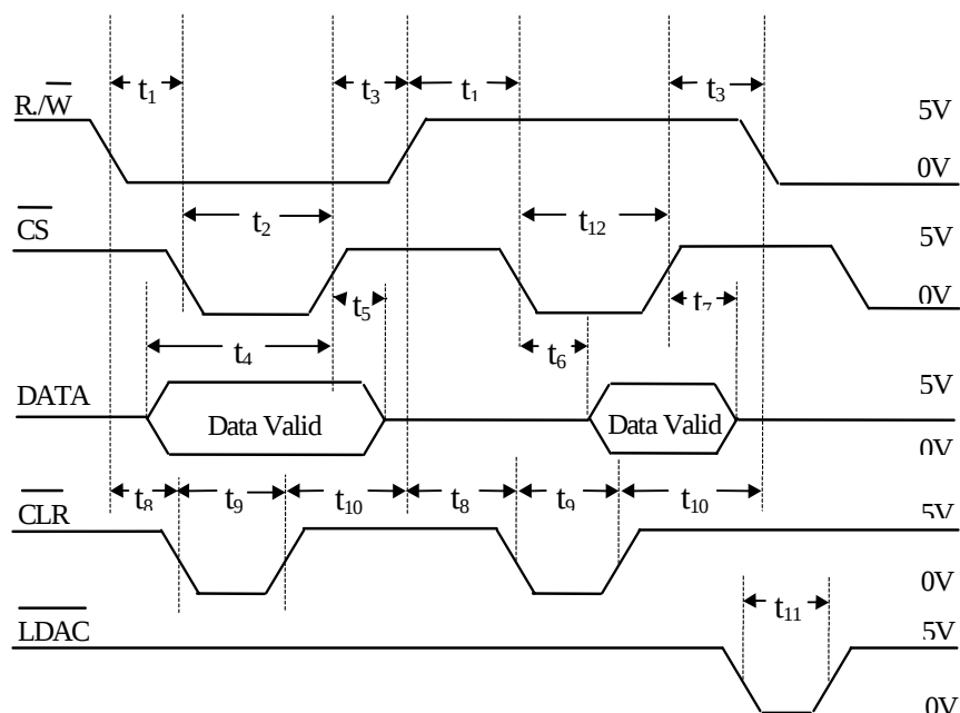
FIGURE 3. 16-BIT DIGITAL TO ANALOG CONVERTER
