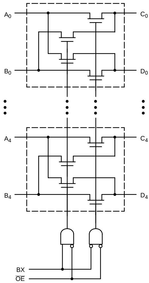
Figure 2. Logic Diagram
