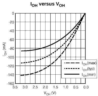
FIGURE 1. Characteristics for Output - Pull Up Driver
