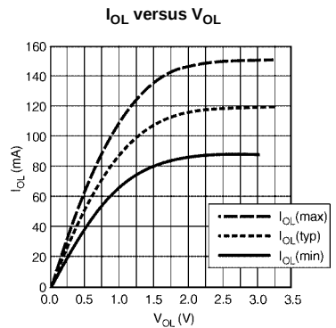
FIGURE 2. Characteristics for Output - Pull Down Driver
