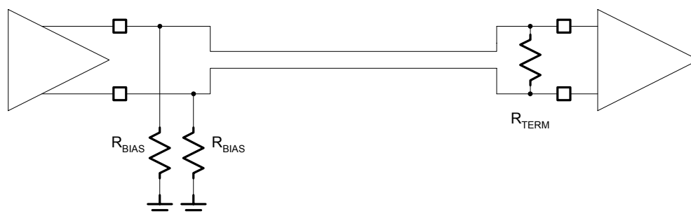
FIGURE 4. PECL INTERFACE
