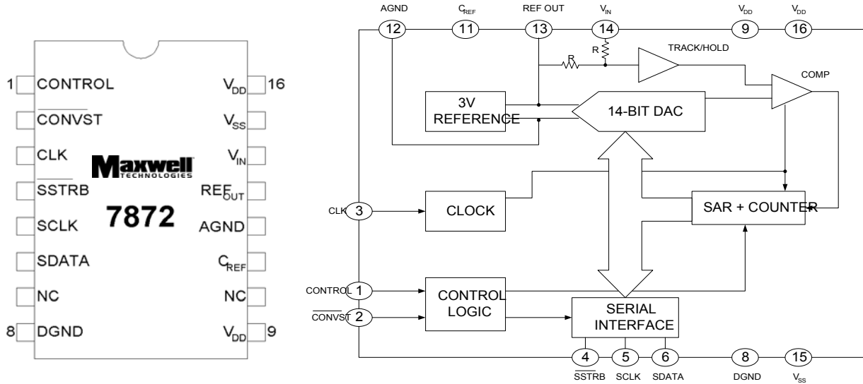
Logic Diagram
