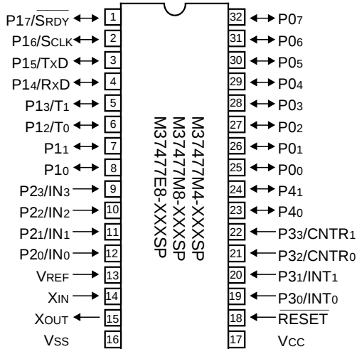
Outline 32P4B (Note 1)
