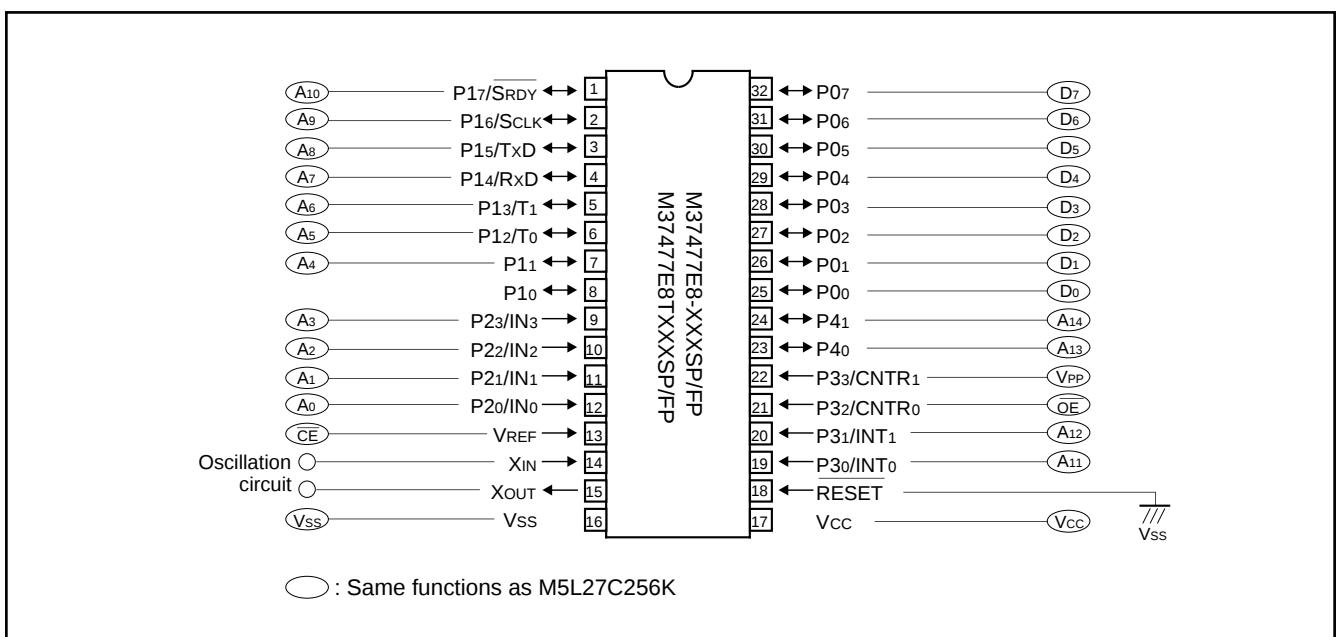
Fig. 32 Pin connection in EPROM mode (7477 Group)
