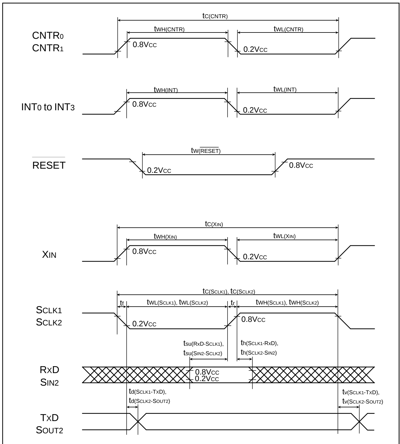
Fig. 81 Timing diagram
