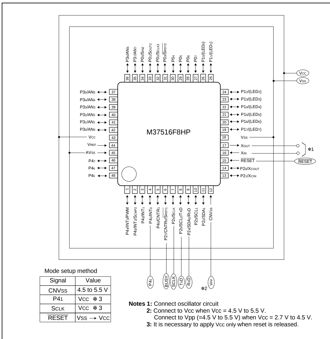
Fig. 65 Pin connection diagram in standard serial I/O mode
