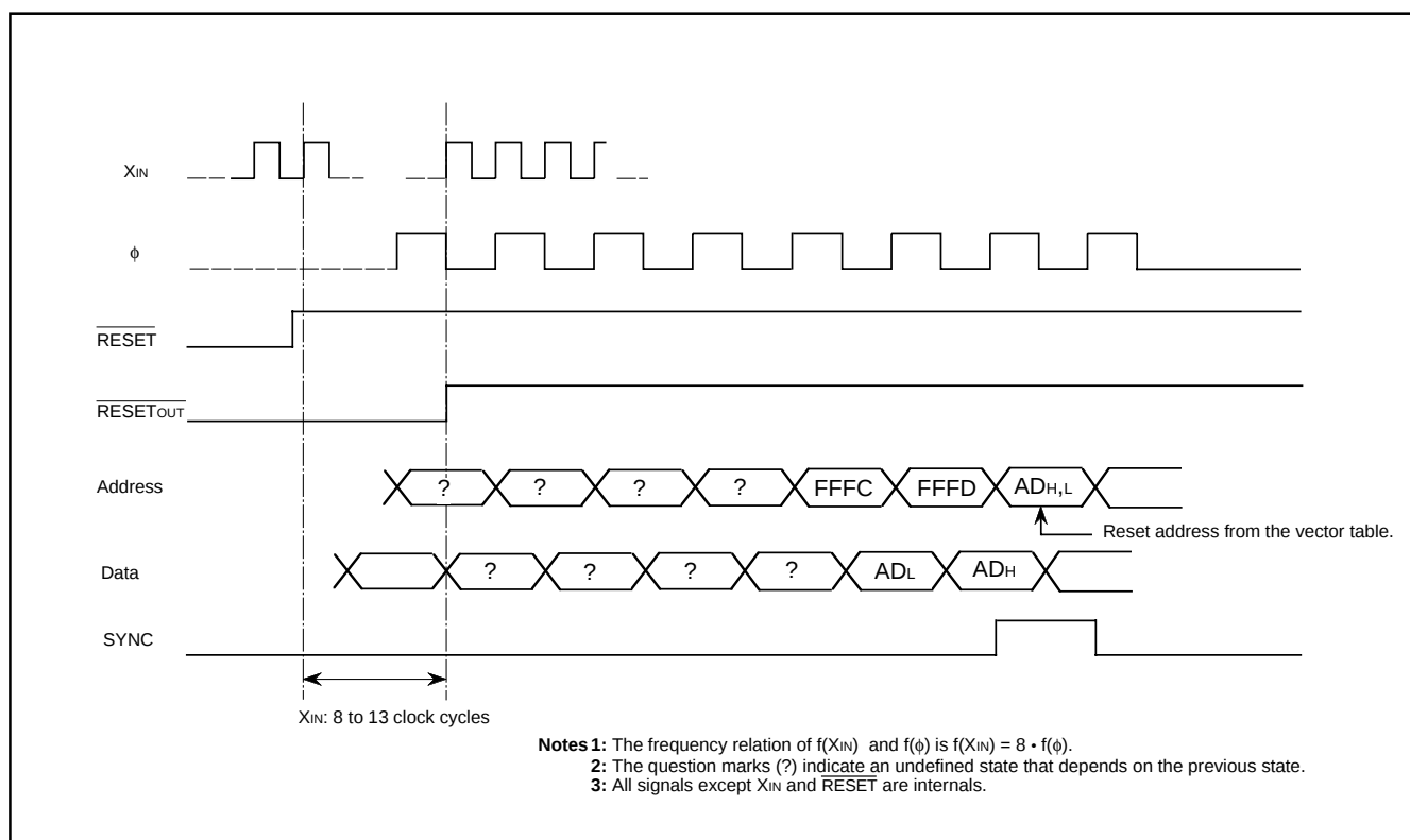
Fig. 50 Reset sequence
