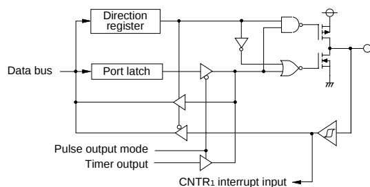
(15) Port P40
