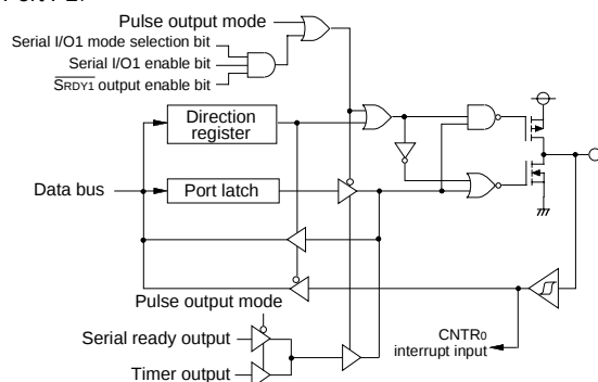
(13) Port P27
