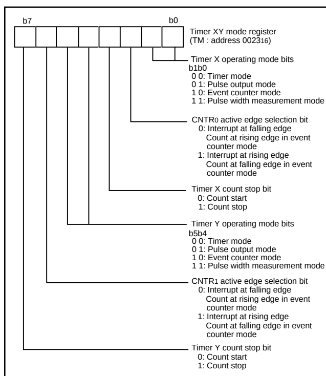
Fig. 15 Structure of timer XY mode register
