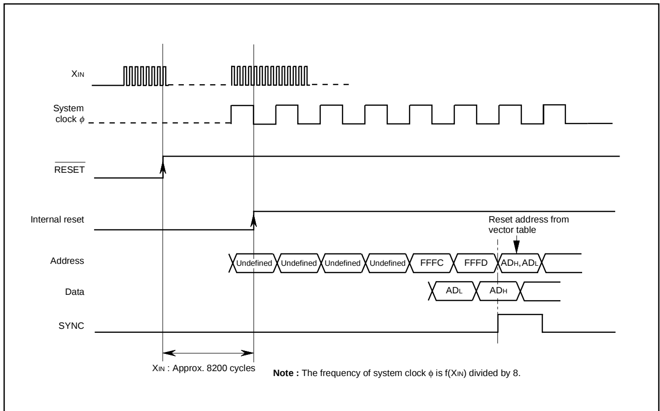
Fig. 55 Reset Sequence
