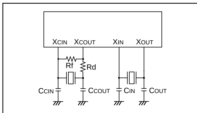
Fig. 57 Oscillator circuit
