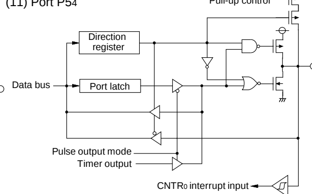
(11) Port P54
