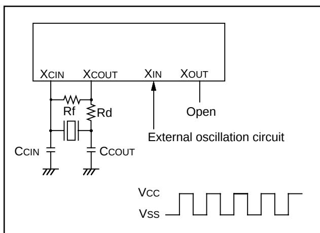
Fig. 58 External clock input circuit
