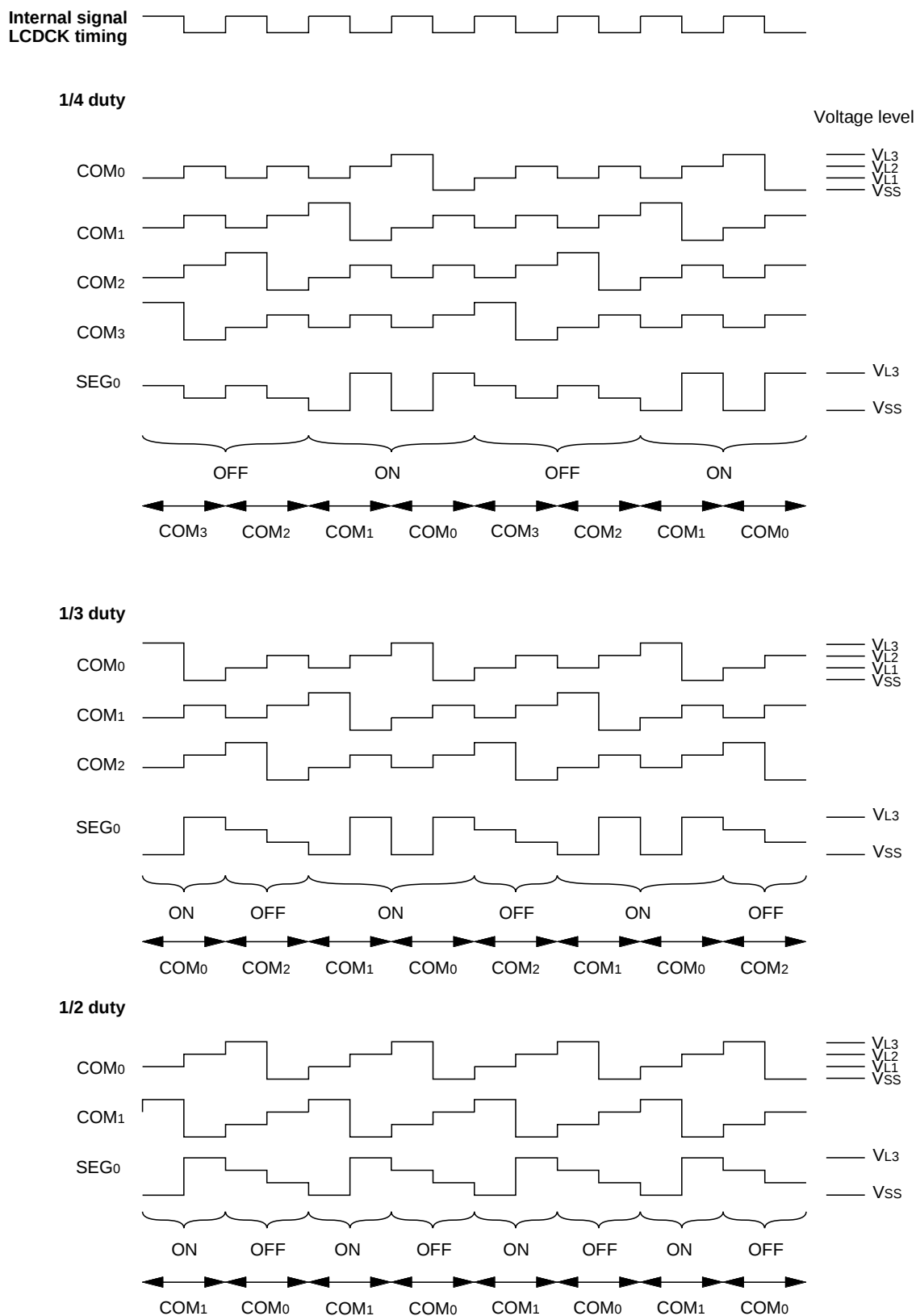
Fig. 49 LCD drive waveform (1/3 bias)
