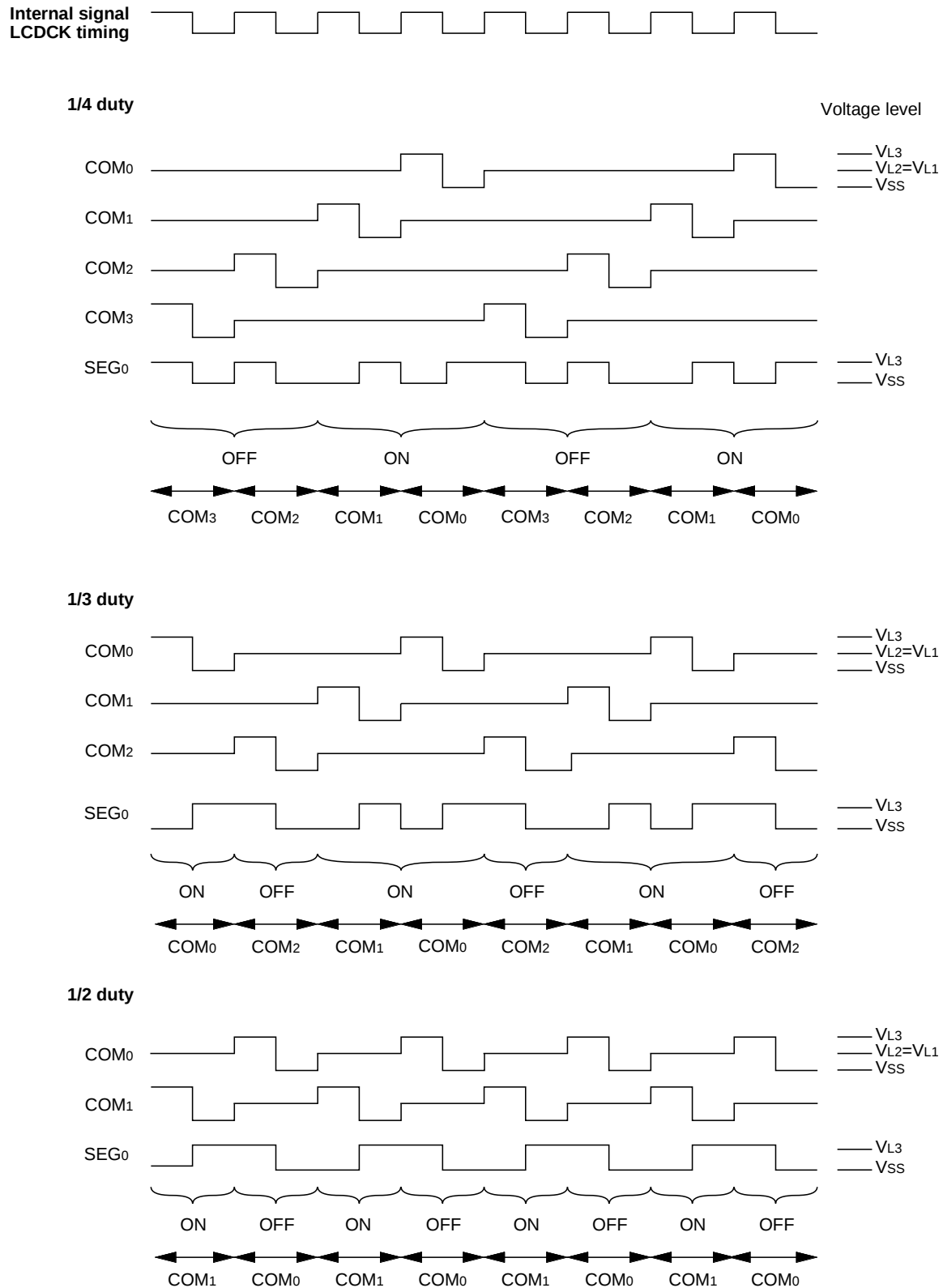
Fig. 48 LCD drive waveform (1/2 bias)
