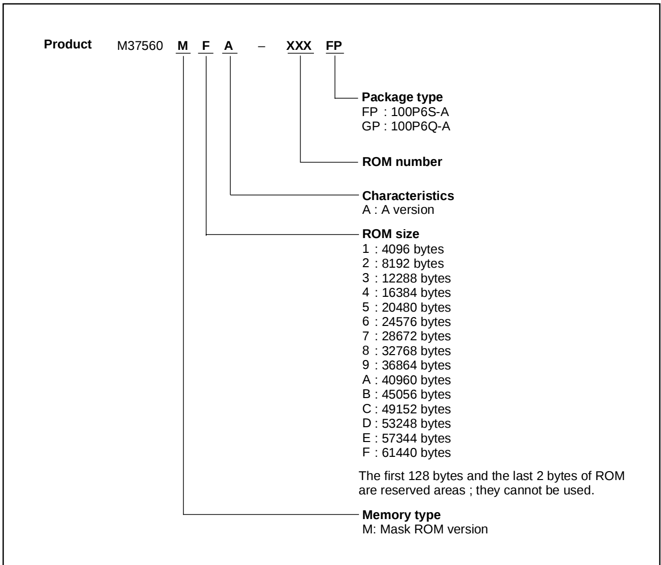
Fig. 4 Part numbering
