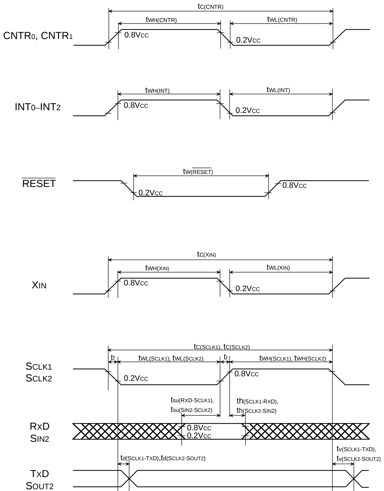
Fig. 66 Timing diagram
