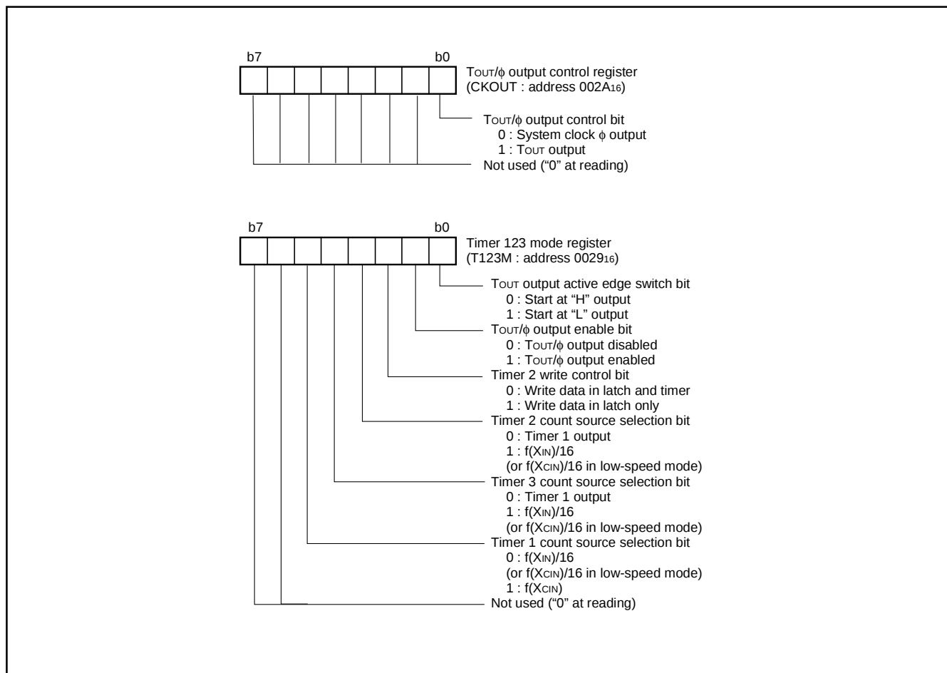
Fig. 53 Structure of TOUT/φ output-related registers
