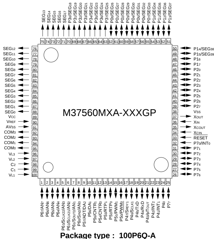
Fig. 2 Pin configuration (Package type: 100P6Q-A)
