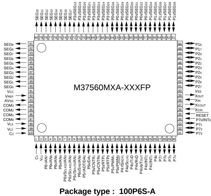
Fig. 1 Pin configuration (Package type: 100P6S-A)
