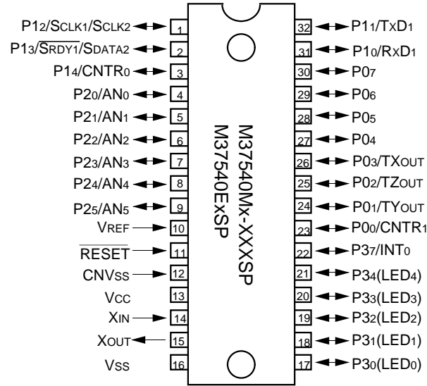
Package type: 32P4B
