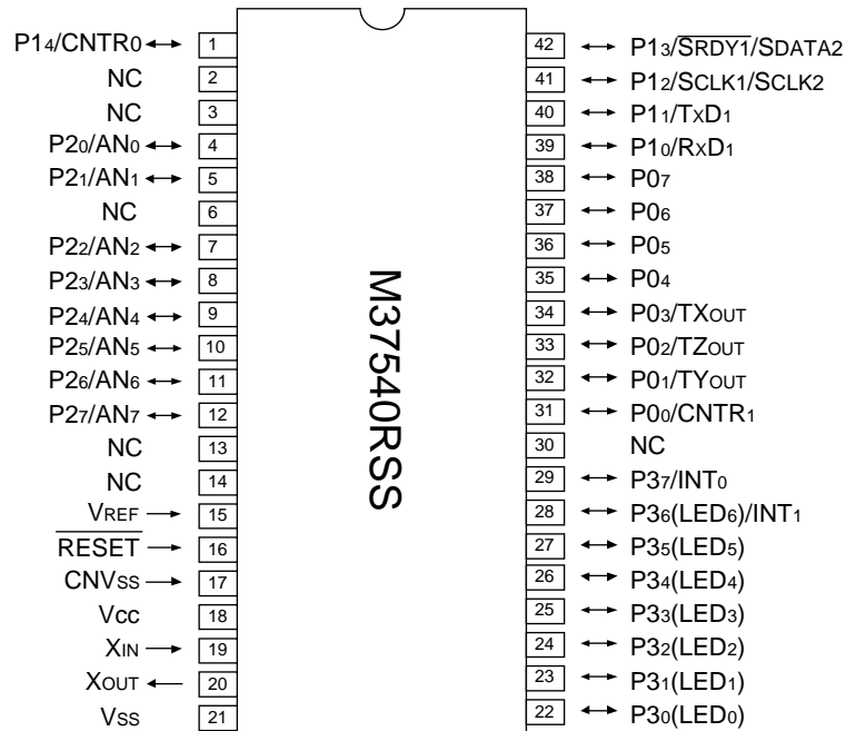
Outline 42S1M
