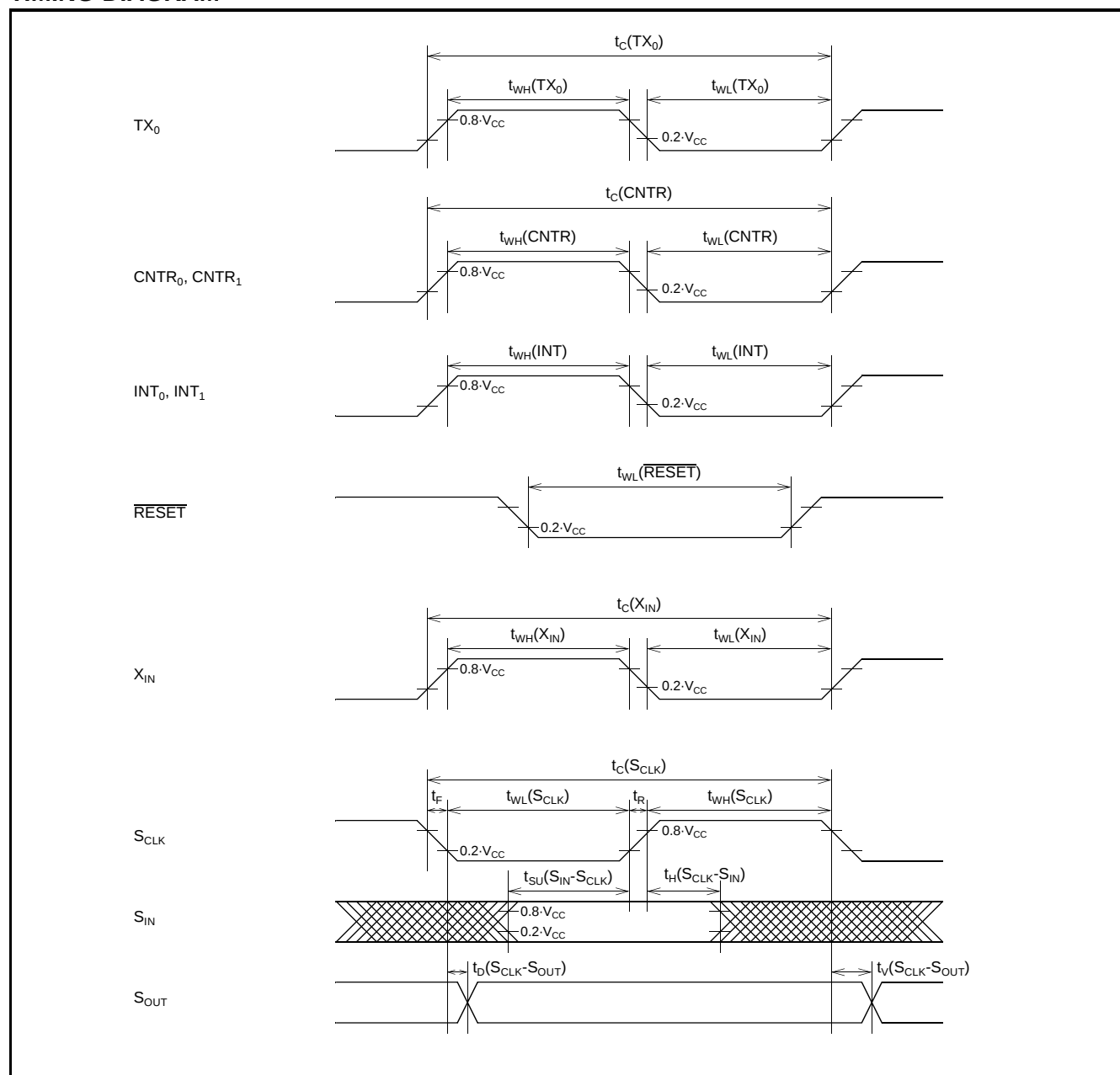
Fig. 50 Timing diagram
