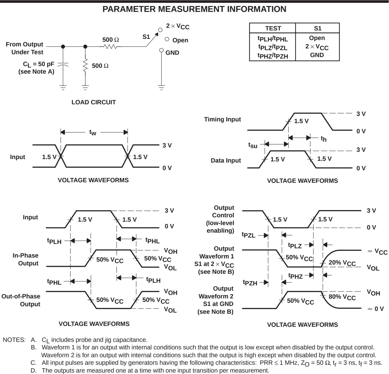
Figure 1. Load Circuit and Voltage Waveforms
