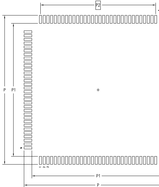
LAND PATTERN DIMENSIONS
