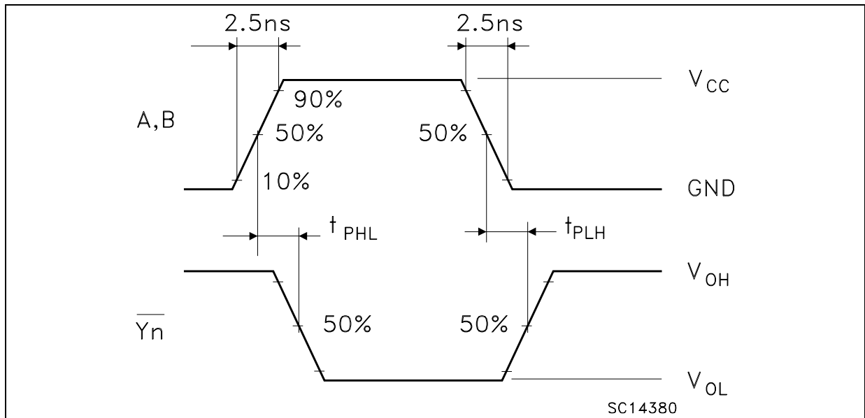
WAVEFORM 1: PROPAGATION DELAYS FOR INVERTING OUTPUTS ( f=1\text{MHz} ; 50% duty cycle)
