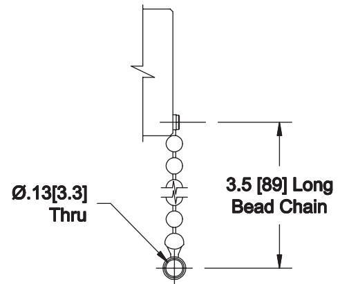
CHAIN DETAIL
