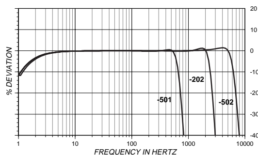
TYPICAL AMPLITUDE RESPONSE
