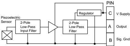
Connection Block Diagram
