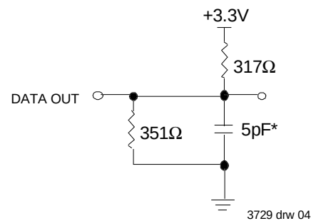
Figure 2. High-Impedance Test Load (for t_{OHZ}, t_{CHZ}, t_{OLZ}, \text{ and } t_{DC1} )
