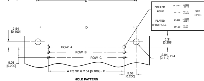
32 contacts, rows a + c even loading
