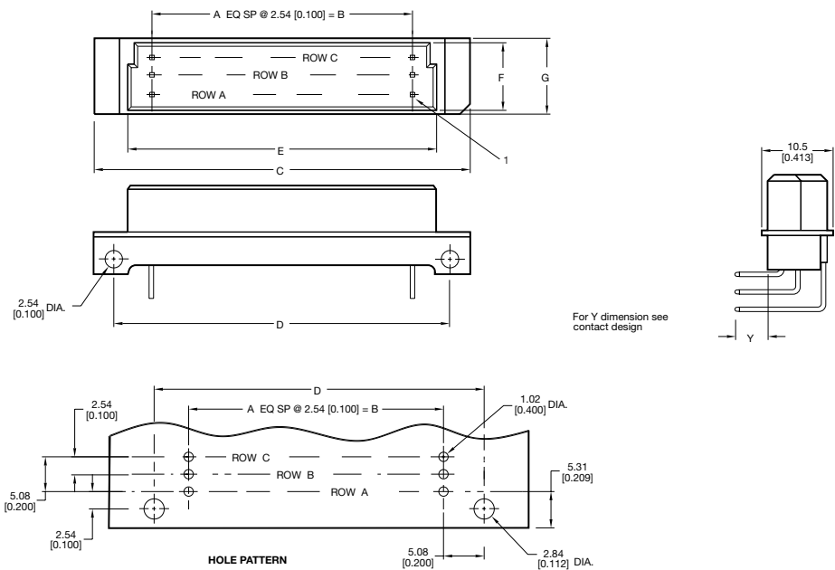
48 contacts, rows a + b + c fully loaded
