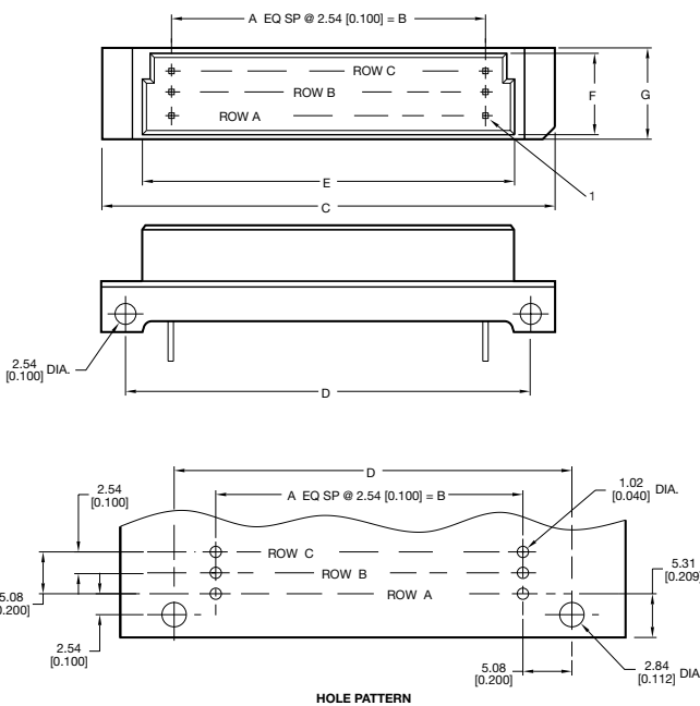
96 contacts, rows a + b + c fully loaded
