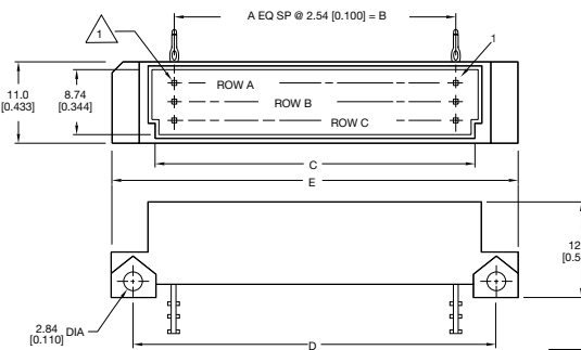
96 contacts, rows a + b + c fully loaded
