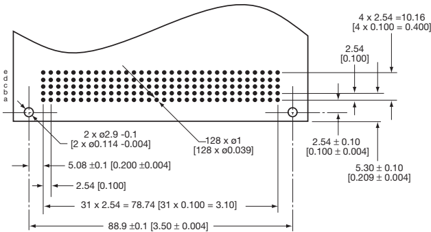
HOLE PATTERN
