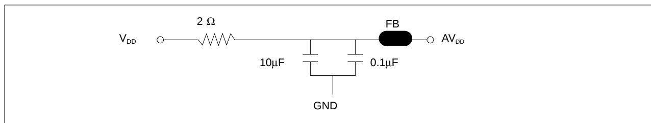
Figure 15. PLL Power Supply Filter Circuit
