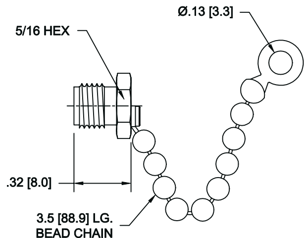
Model Number: 7007C SMA Female with Chain
